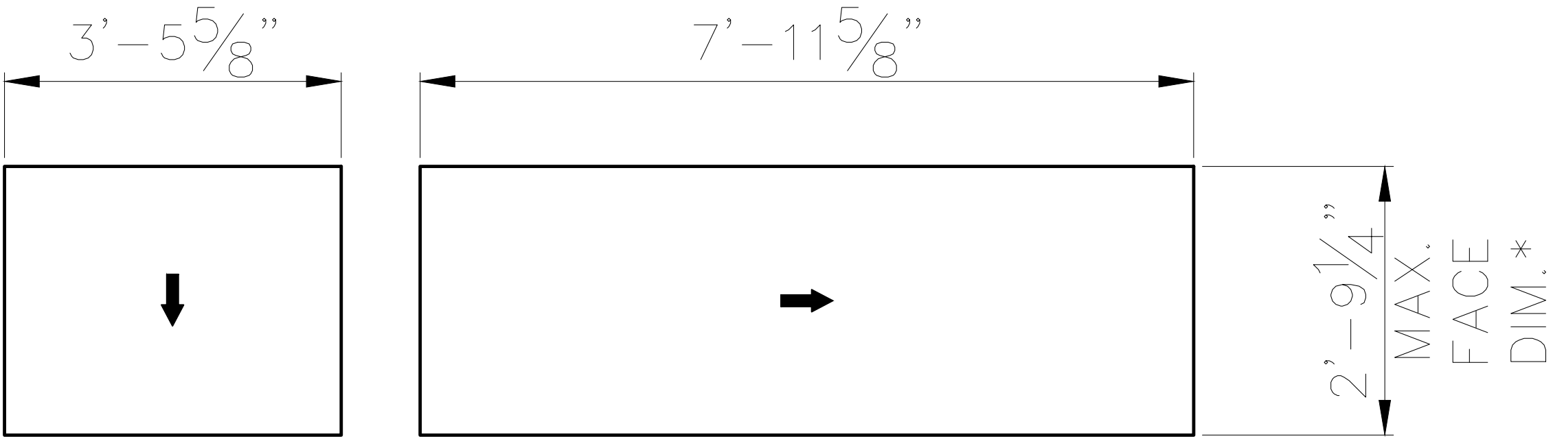
PANEL DRAWINGS SCALE: NONE
