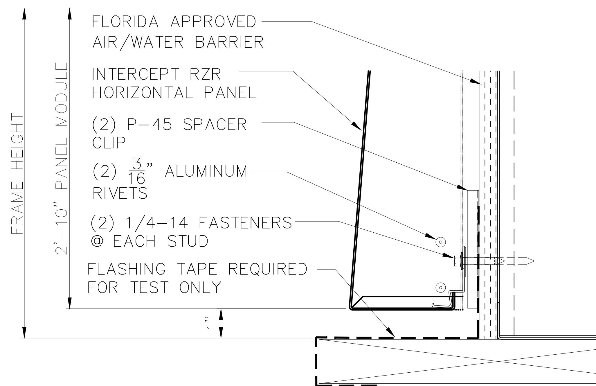
3.2 BASE INTERCEPT RZR PANEL TOP-BOTTOM SLOPE. SCALE: NONE
