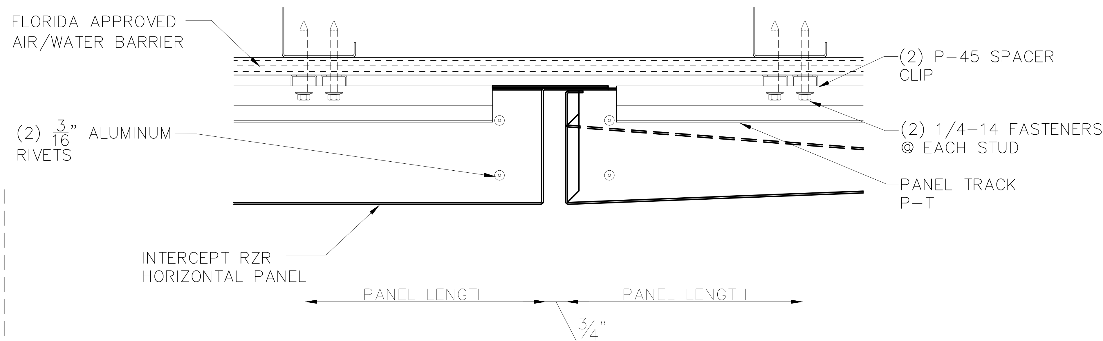
4.2 VERTICAL PANEL JOINT INTERCEPT RZR PANEL TOP-BOTTOM & LEFT-RIGHT SLOPES. SCALE: NONE
