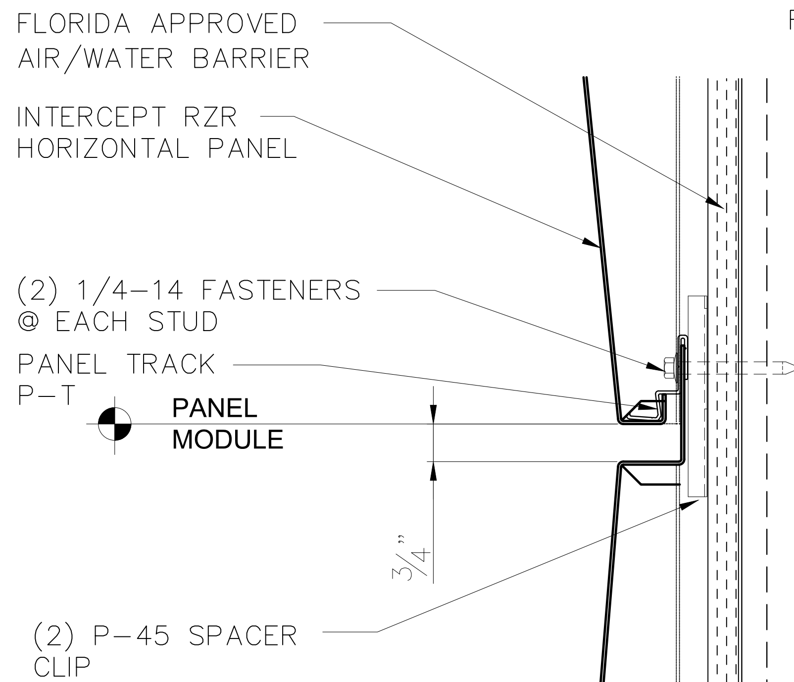
2.2 HORIZONTAL PANEL JOINT INTERCEPT RZR PANEL TOP-BOTTOM SLOPE. SCALE: NONE
