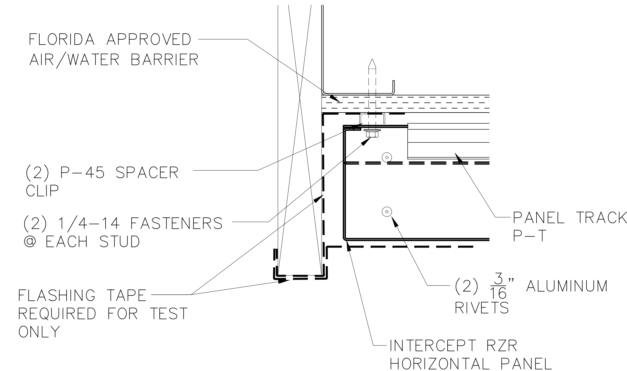
5.2 JAMB INTERCEPT RZR PANEL TOP-BOTTOM SLOPE. SCALE: NONE
